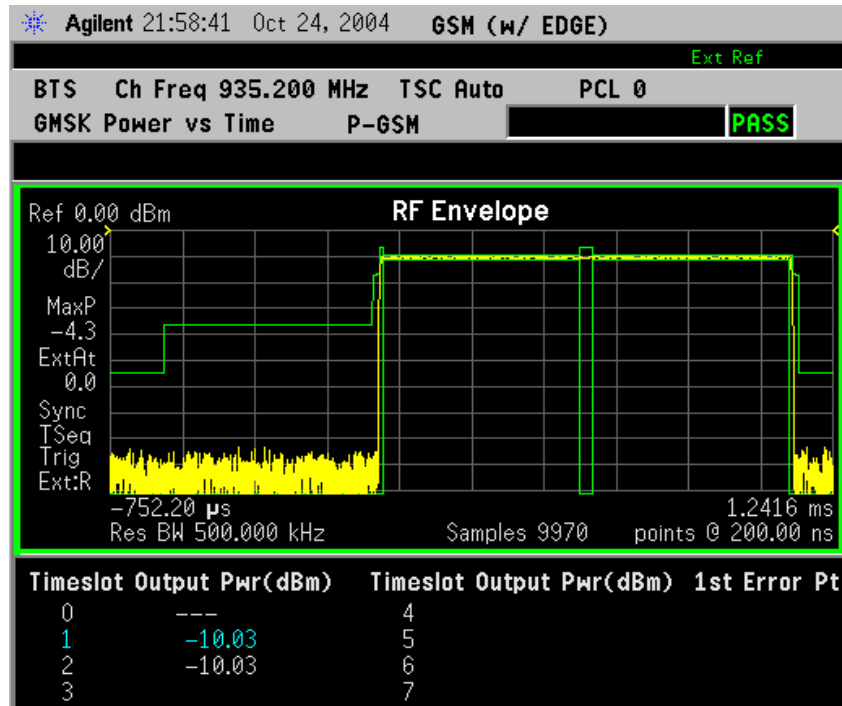
Figure 2-43 GMSK PvT Result - Custom Limit Mask Example of Two Consecutive Bursts
