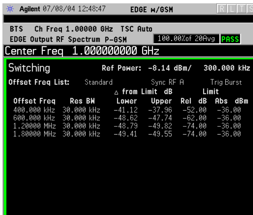
Figure 2-14 EDGE ORFS Result - Switching Margin & Limits View
