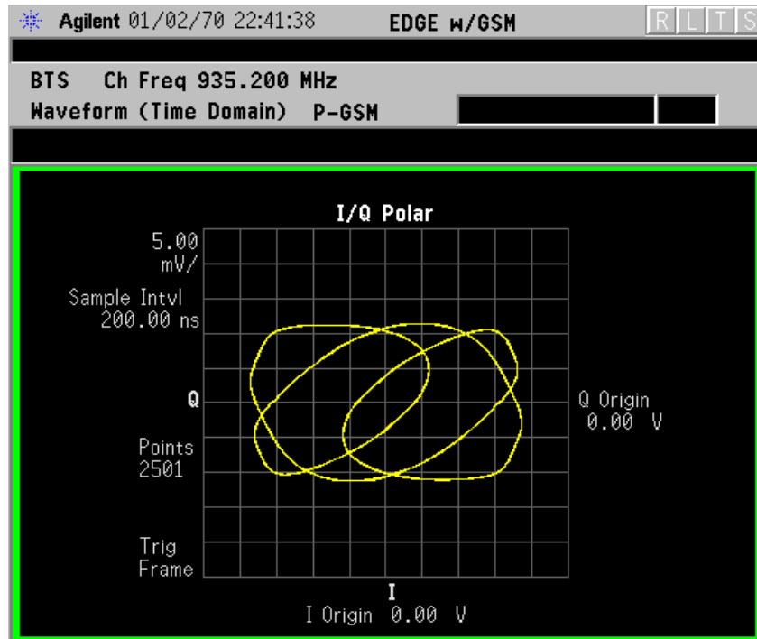
Figure 2-75 Waveform Measurement - I/Q Polar View
