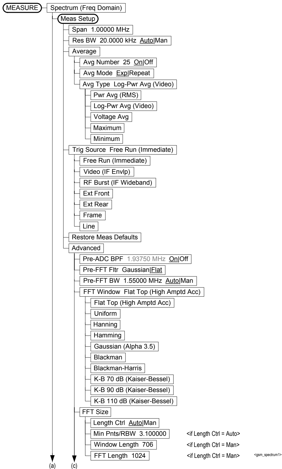
Figure 6-20 Spectrum (Freq Domain) Measurement Key Flow (1 of 3)
