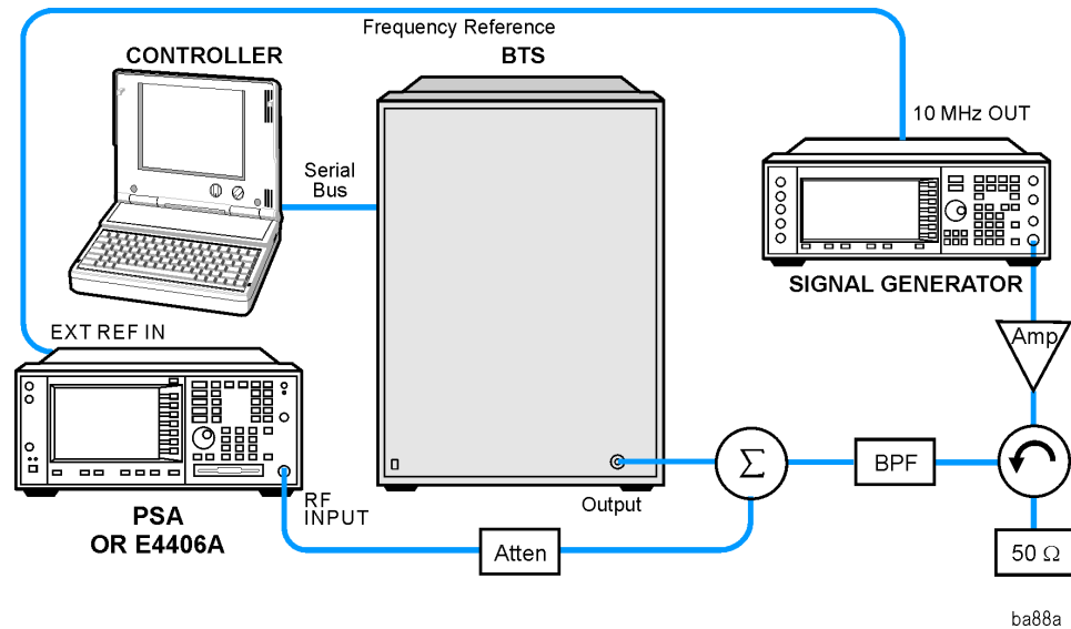
Spectrum Measurement System
