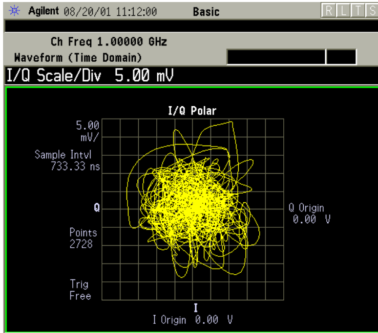
Figure 2-75 Waveform Measurement - I/Q Polar View
