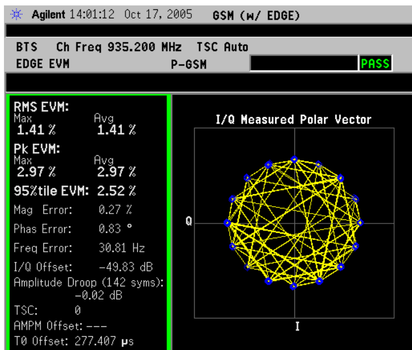
Figure 2-7 EDGE EVM Result - Polar Vector View
