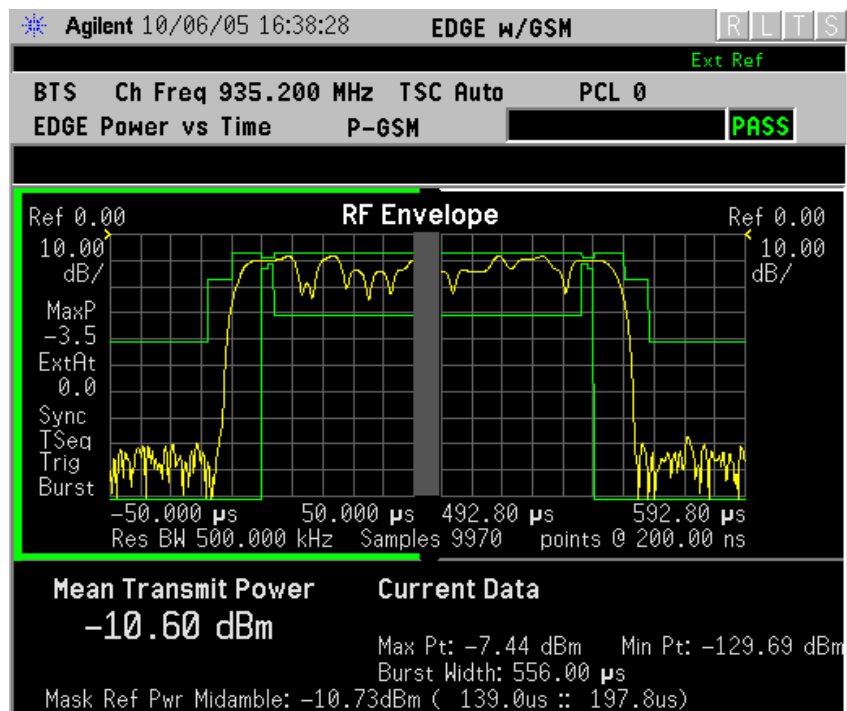
Figure 2-3 EDGE Power vs. Time Result - Rise & Fall View
