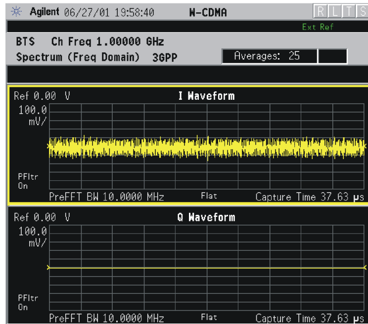
Figure 2-51 Spectrum Measurement - I and Q Waveform View (for E4406A)
