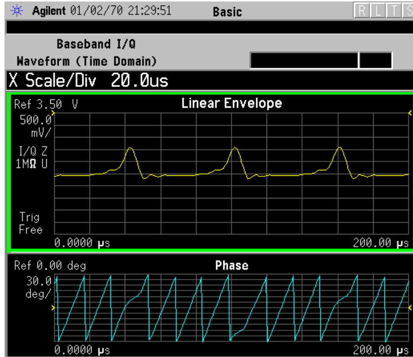
Figure 2-65 Waveform Measurement - Linear Envelope View
